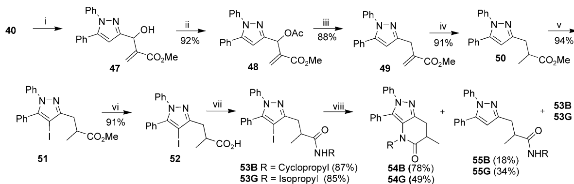
Scheme 8. Reaction conditions: i) Ref. [6] ii) AcCl (1.5 equiv.), pyridine (1.3 equiv.), CH 2 Cl 2 , 0°C to room temperature, 2 h. iii) 1) DABCO (1 equiv.), THF-H 2 O (1:1, v/v), room temperature, 15 min; 2) NaBH 4 (1 equiv.), room temperature, 30 min. iv) Raney-Ni, H 2 , MeOH, 40 psi, room temperature, 3 h. v) ICl (3 equiv.), K 2 CO 3 (3 equiv.), CHCl 3 , room temperature, 12 h. vi) Aqueous LiOH (5 equiv.), THF-MeOH (5:1, v/v), room temperature, 5 h. vii) 1) Isobutyl chloroformate (1.5 equiv.), NMM (1.5 equiv.), THF, -10°C, 15 min; 2) RNH 2 (1.2 equiv.), THF, -10°C, 30 min. viii) CuI (0.2 equiv.), NH 2 (CH 2 ) 2 NH 2 (0.4 equiv.), Cs 2 CO 3 (2 equiv.), DMF, 100°C, 48 h (yields of 54 and 55 are based on the consumed starting material).
