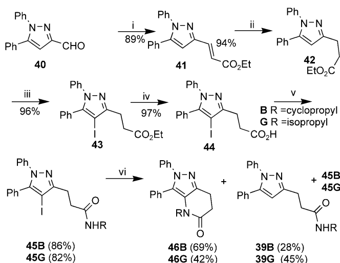
Scheme 7. Reaction conditions: i) (EtO) 2 P(O)CH 2 CO 2 Et (1.5 equiv.), NaH (3 equiv.), THF, 0°C to room temperature, 4 h. ii) Raney-Ni, H 2 , EtOH, 40 psi, room temperature, 3 h. iii) ICl (3 equiv.), K 2 CO 3 (3 equiv.), CHCl 3 , room temperature, 10 h. iv) Aqueous LiOH (5 equiv.), THF-MeOH (5:1, v/v), room temperature, 5 h. v) 1) Isobutyl chloroformate (1.5 equiv.), NMM (1.5 equiv.), THF, -10°C, 20 min; 2) RNH 2 (1.2 equiv.), -10°C, 30 min. vi) CuI (0.2 equiv.), NH 2 (CH 2 ) 2 NH 2 (0.4 equiv.), Cs 2 CO 3 (2 equiv.), DMF, 100°C, 48 h (yields of 46 and 39 are based on the consumed starting material).
