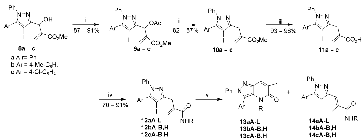
Scheme 2. Reactions conditions: i) AcCl (1.5 equiv.), pyridine (1.3 equiv.), CH 2 Cl 2 , 0°C to room temperature, 2 h. ii) 1) DABCO (1 equiv.), THF-H 2 O (1:1, v/v), room temperature, 15 min; 2) NaBH 4 (1 equiv.), room temperature, 30 min. iii) Aqueous LiOH (5 equiv.), THF-MeOH, (5:1, v/v), room temperature, 5 h. iv) 1) DCC (1 equiv.), HOBT (1 equiv.), DMF, room temperature, 30 min; 2) RNH 2 (1.1 equiv.), 2 h. v) CuI (0.2 equiv.), NH 2 (CH 2 ) 2 NH 2 (0.4 equiv.), Cs 2 CO 3 (2 equiv.), DMF, 100°C, 24 h.
