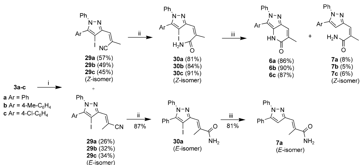
Scheme 4. Reaction conditions: i) NaBH 4 (1.2 equiv.), MeOH, 0°C, 20 min. ii) TFA-H 2 SO 4 (1:1, v/v), room temperature, 6–8 h. iii) CuI (0.2 equiv.), NH 2 (CH 2 ) 2 NH 2 (0.4 equiv.), Cs 2 CO 3 (2 equiv.), DMF, 100°C, 18 h [for 30 (Z-isomer)] and 24 h [for 30 (E-isomer)].
