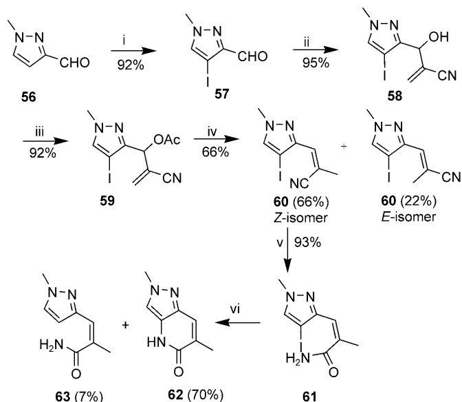
Scheme 9. Reaction conditions: i) ICl (3 equiv.), K 2 CO 3 (3 equiv.), CHCl 3 , room temperature, 10 h. ii) CH 2 =CHCN, (1.1 equiv.), DABCO (1 equiv.), room temperature, 4 h. iii) AcCl (1.5 equiv.), pyridine (1.3 equiv.), CH 2 Cl 2 , 0°C to room temperature, 2 h. iv) NaBH 4 (1.2 equiv.), MeOH, room temperature, 20 min. v) TFA-H 2 SO 4 (1:1, v/v), room temperature, 10 h. vi) CuI (0.2 equiv.), NH 2 (CH 2 ) 2 NH 2 (0.4 equiv.), Cs 2 CO 3 (2 equiv.), DMF, 100°C, 18 h.
