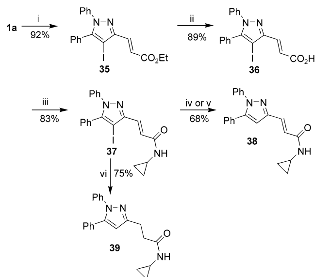
Scheme 6. Reaction conditions: i) (EtO) 2 P(O)CH 2 CO 2 Et (1.5 equiv.), NaH (3 equiv.), THF, 0°C to room temperature, 4 h. ii) Aqueous LiOH (5 equiv.), THF-MeOH (5:1, v/v), room temperature, 5 h. iii) 1) DCC (1 equiv.), HOBT (1 equiv.), DMF, room temperature, 30 min; 2) cyclopropylamine (1.1 equiv.), room temperature, 2 h. iv) CuI (0.2 equiv.), NH 2 (CH 2 ) 2 NH 2 (0.4 equiv.), Cs 2 CO 3 (2 equiv.), DMF, 100°C, 24 h. v) Et 3 SiH, PdCl 2 , EtOH, room temperature, 24 h or Pd-C, H 2 , 40 psi, 3 h. vi) Raney-Ni, H 2 , MeOH, 40 psi, 3 h.
