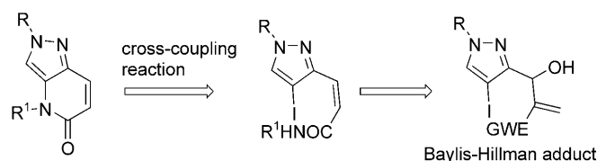
Figure 1. Retrosynthetic pathway for pyrazolo[4,3- b ]pyridine-5-ones.
