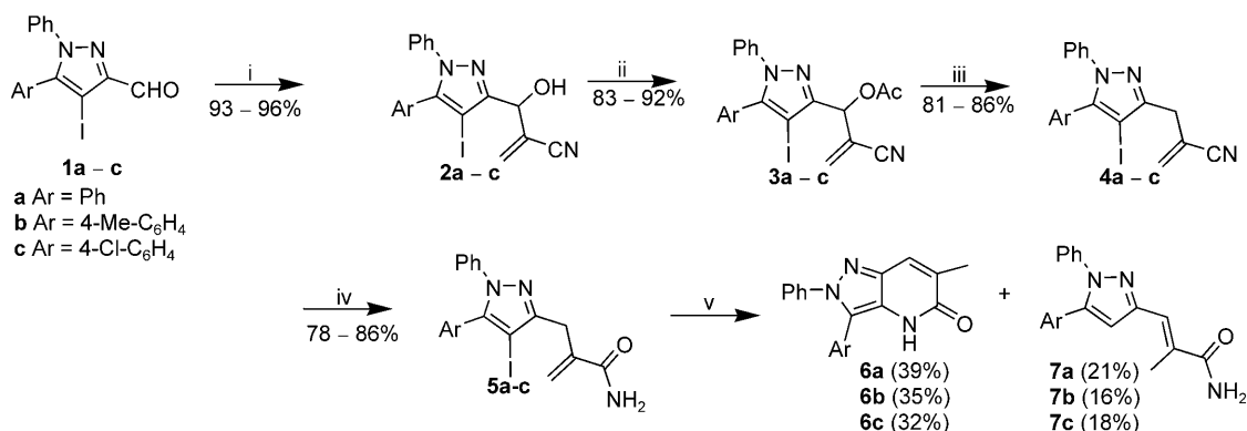
Scheme 1. Reaction conditions: i) Ref. [6] ii) AcCl (1.5 equiv.), pyridine (1.3 equiv.), CH 2 Cl 2 , 0 °C to room temperature, 2 h. iii) 1) DABCO (1 equiv.), THF–H 2 O (1:1, v/v), room temperature, 15 min; 2) NaBH 4 (1 equiv.), room temperature, 30 min. iv) TFA–H 2 SO 4 (1:1, v/v), room temperature, 4 h. v) CuI (0.2 equiv.), NH 2 (CH 2 ) 2 NH 2 (0.4 equiv.), Cs 2 CO 3 (2 equiv.), DMF, 100 °C, 24 h.
