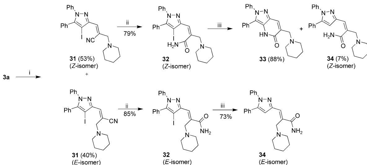
Scheme 5. Reaction conditions: i) Piperidine (1 equiv.), MeOH, room temperature, 1 h. ii) TFA-H 2 SO 4 (1:1, v/v), room temperature, 8 h. iii) CuI (0.2 equiv.), NH 2 (CH 2 ) 2 NH 2 (0.4 equiv.), Cs 2 CO 3 (2 equiv.), DMF, 100°C, 18 h [for 32 (Z-isomer)] and 24 h [for 32 (E-isomer)].
